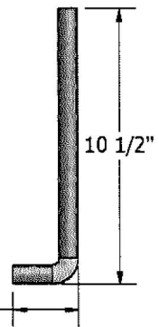
J-BOLT DETAIL
