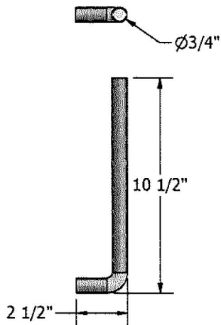
J-BOLT DETAIL
