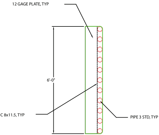
END/ELEVATION VIEW
