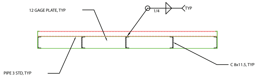
SIDE/ELEVATION VIEW
